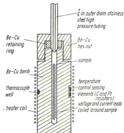
Fig. 1. Sample chamber and high pressure bomb details
